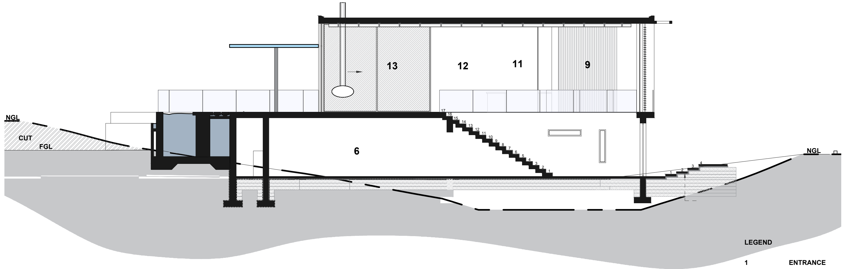
SECTION D-D SCALE 1:100
